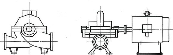
图 C.19 中开泵
